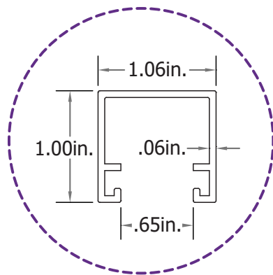
Top, Middle, & Bottom Rails
